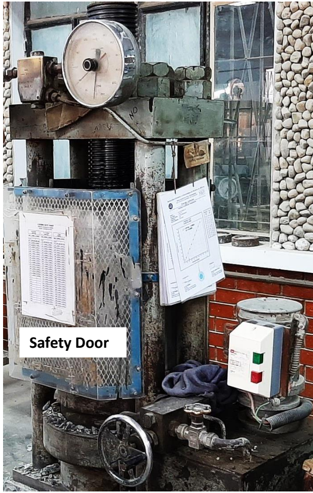
Manual Concrete compression machine
